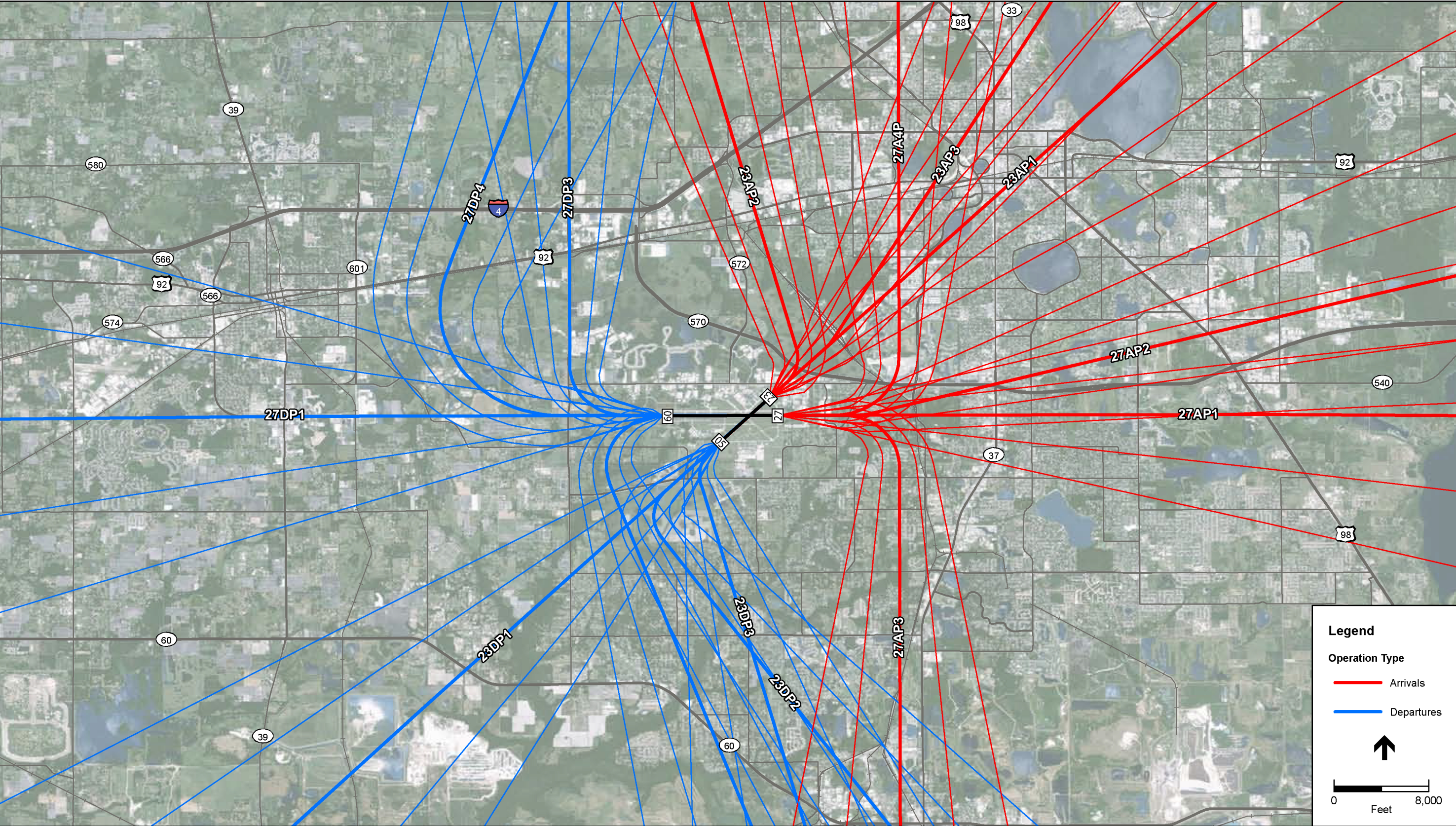
SOURCE: AEDT 2b SP2; ESA Airports, 2016 Lakeland Linder Regional Airport MRO Environmental Assessment.150755 Figure 2 West Flow Itinerant AEDT Flight Tracks
