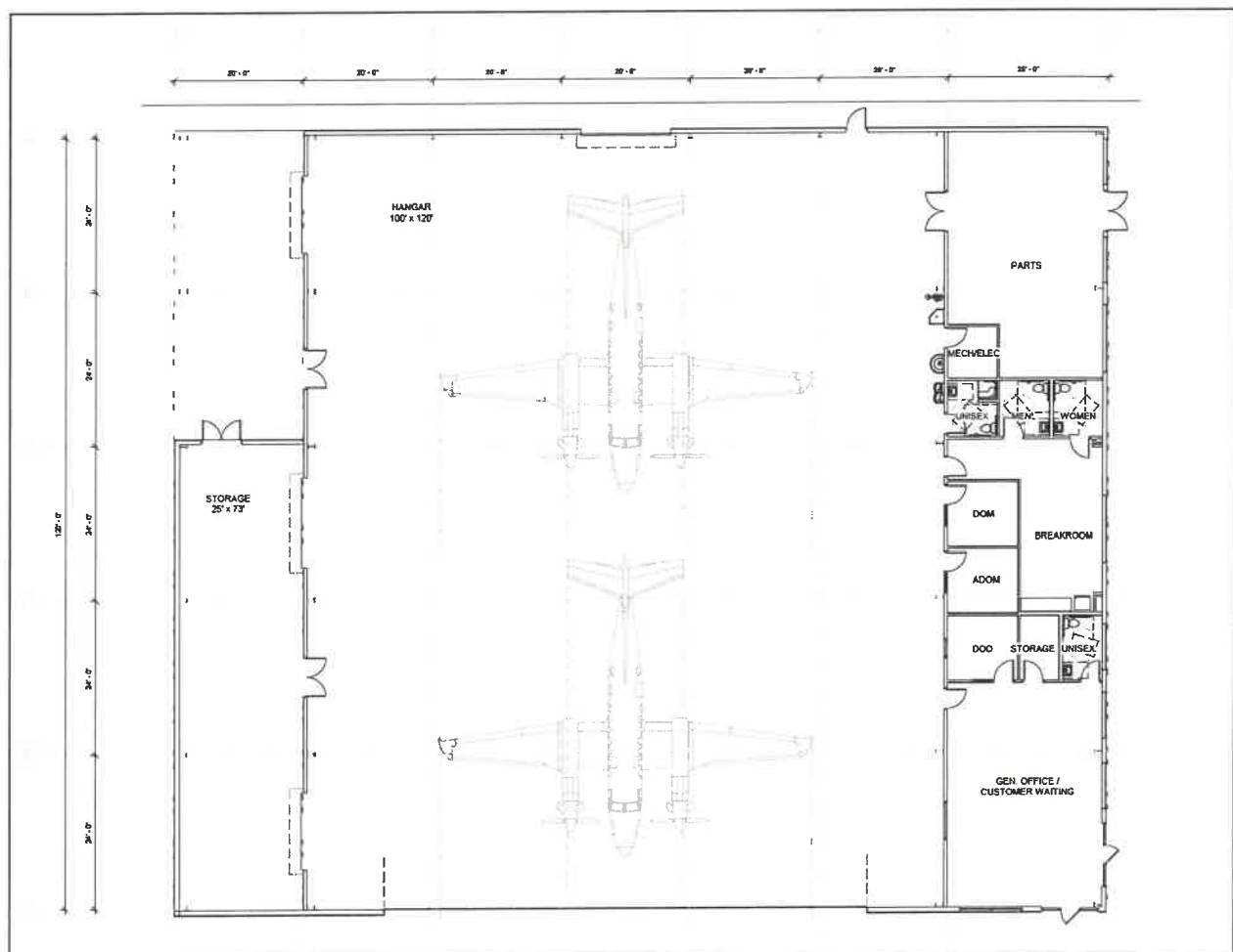
FIGURE 1: PROPOSED HANGAR / OFFICE / STORAGE LAYOUT
